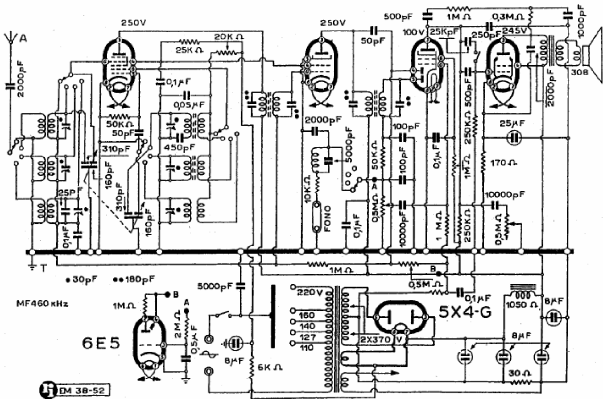
Watt Radio - Mod. 6L6 Taurus Fono
